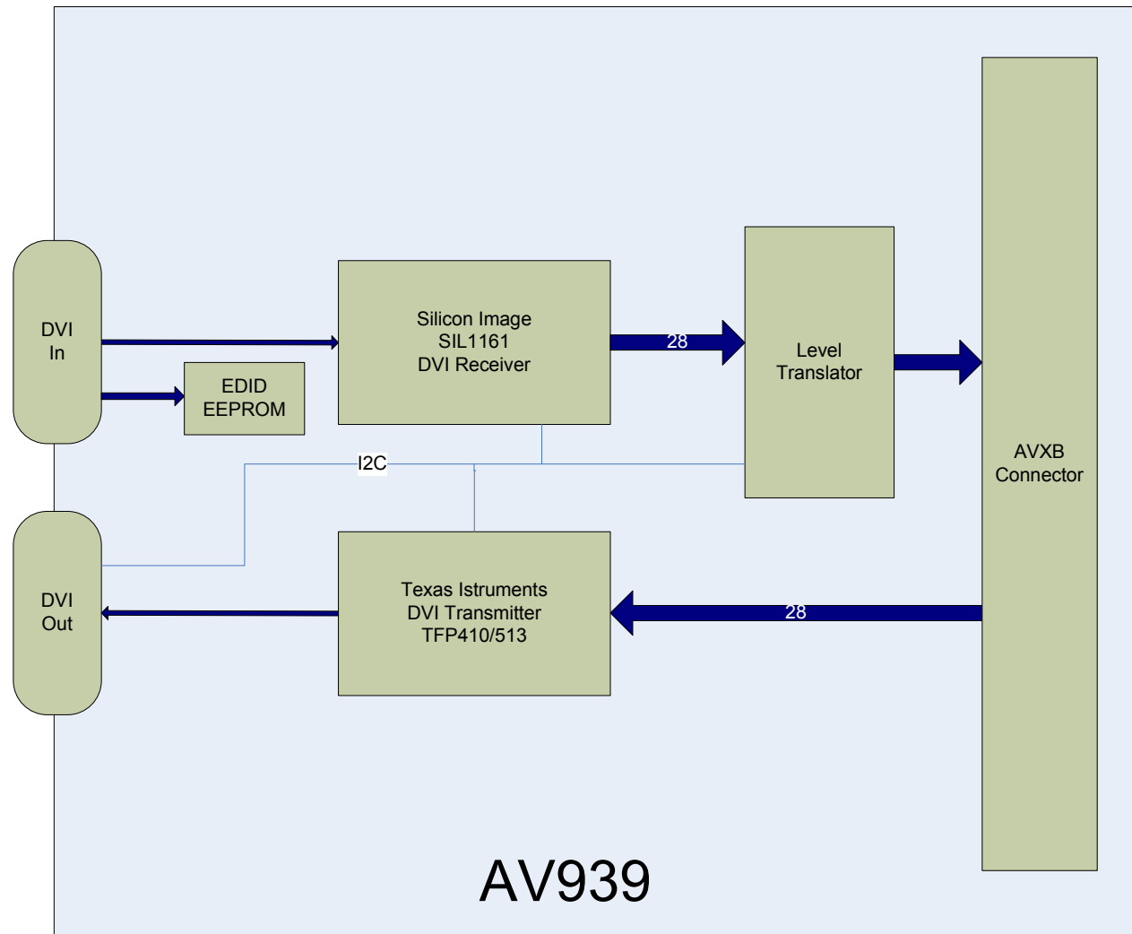
Figure 1 : AV939 Block Diagram
