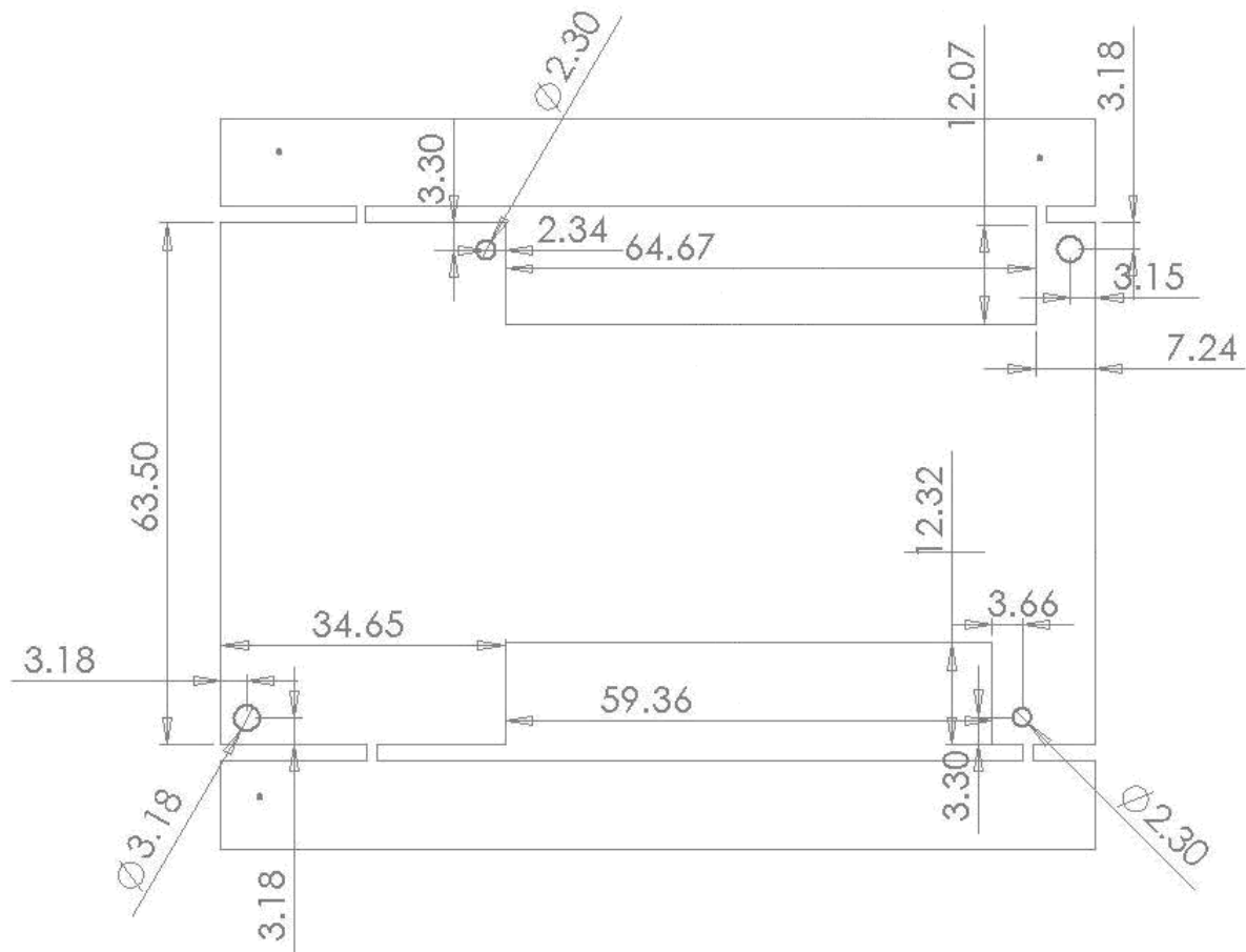
Figure 2 – Board Dimensions
